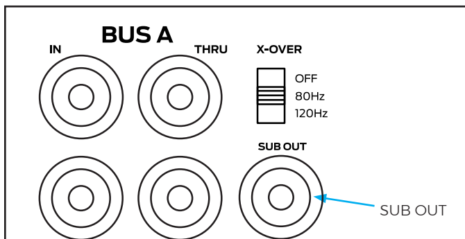
Figure 4: Using the Subwoofer Line-Level Output with the Bus A Inputs (not applicable with the Bus B or local inputs)
