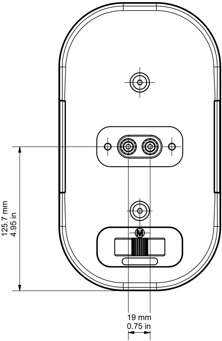
REAR VIEW
